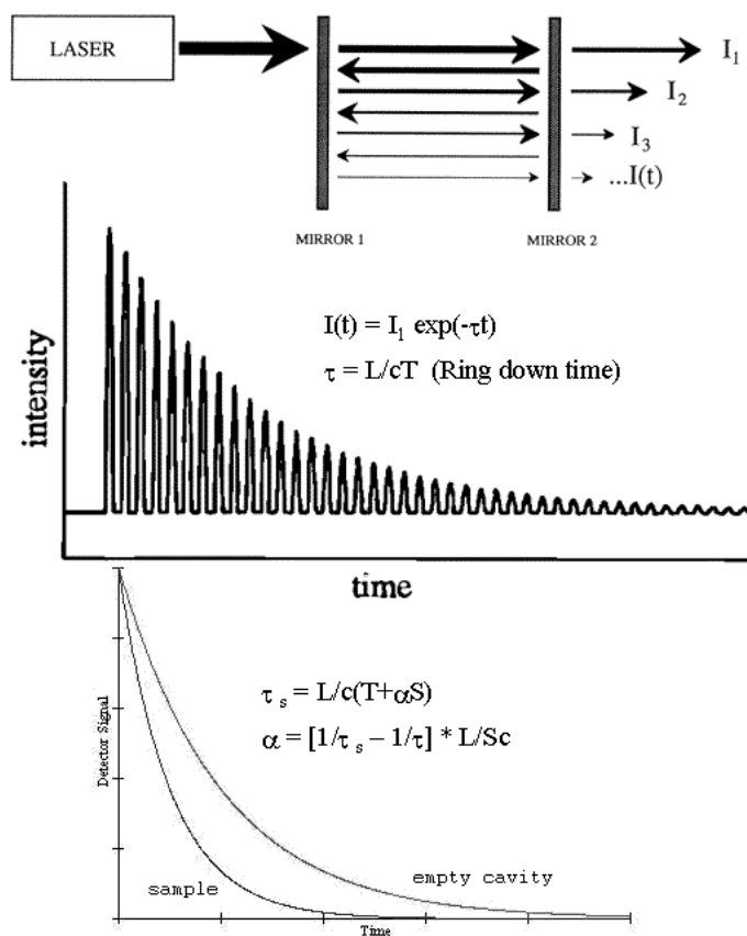
Figure 1. Cavity Ring down spectroscopy scheme.
