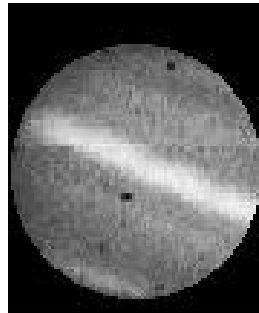
Figure 1. K' band image of Jupiter observed on 25 Dec 2003, 00:25 UT using NICMOS in imaging mode.
