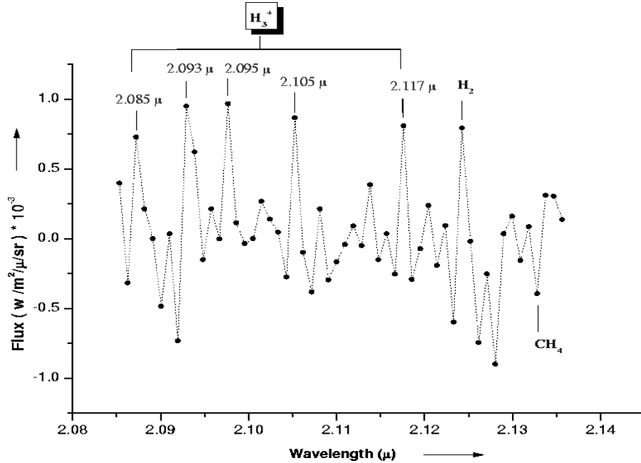
Figure 2. Figure shows a portion of the K' band spectrum of Jupiter taken in the northern auroral zone 306 deg long on 25 Dec 2003 at 23:00 UT. A continuum has been subtracted from the spectra which was then ratioed with a nearby standard star spectrum ( \theta Leonis, A2 type) to remove terrestrial atmospheric absorption. Line flux calibration has been done using 2MASS K magnitude of the star and a blackbody temperature of 9380 K.
