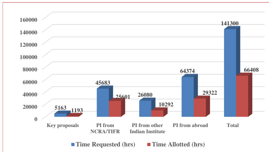
GMRT Proposal Statistics - Cycle 1 to Cycle 38 Time Requested Vs Time Allotted
